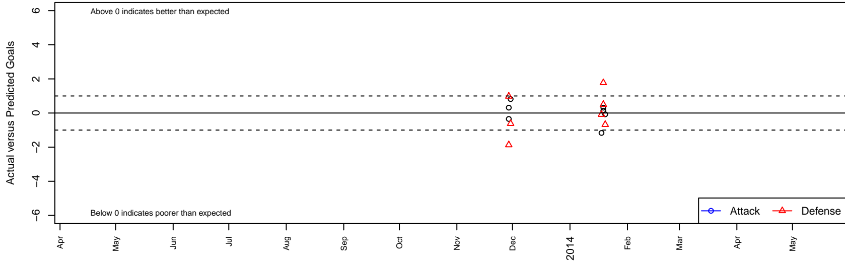
Alaska YS B96 Dots are actual minus expected GF (blue circles) and GA (red triangles). Blue line is smoothed change in attack strength. Red is smoothed change in defense strength.
